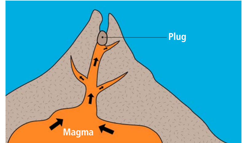
Some volcanoes become plugged (above), and then they explode violently (below).
