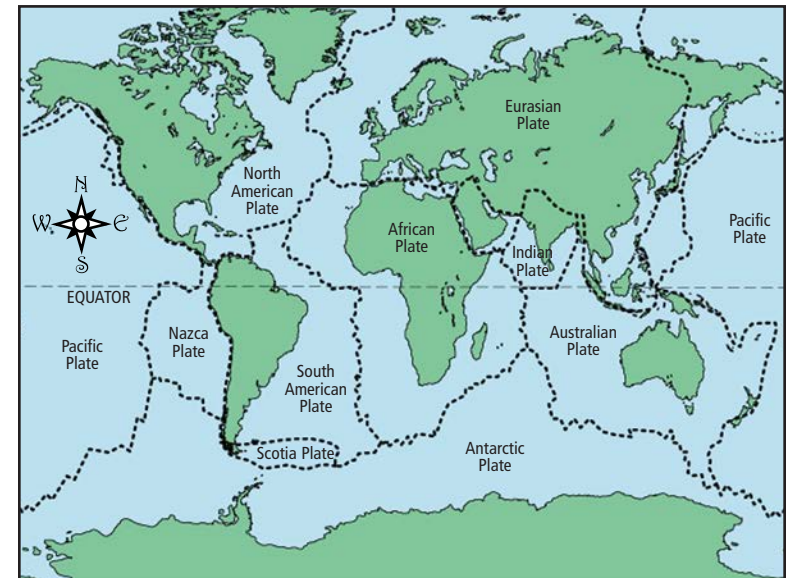
The dotted lines show the edges of the tectonic plates.
